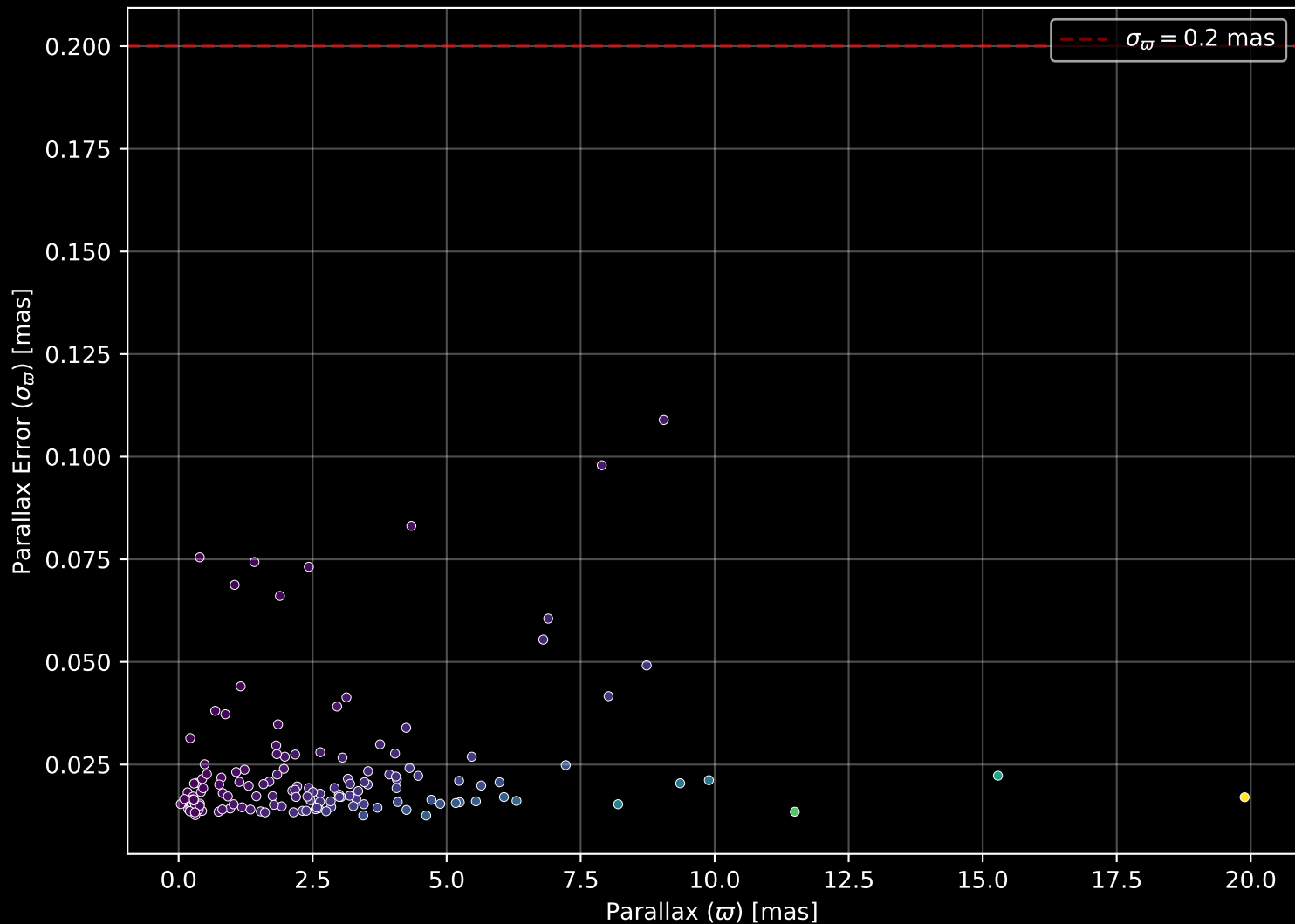
APOGEE DR17 Field: [042-31_MGA] Parallax Quality (n= 149)
