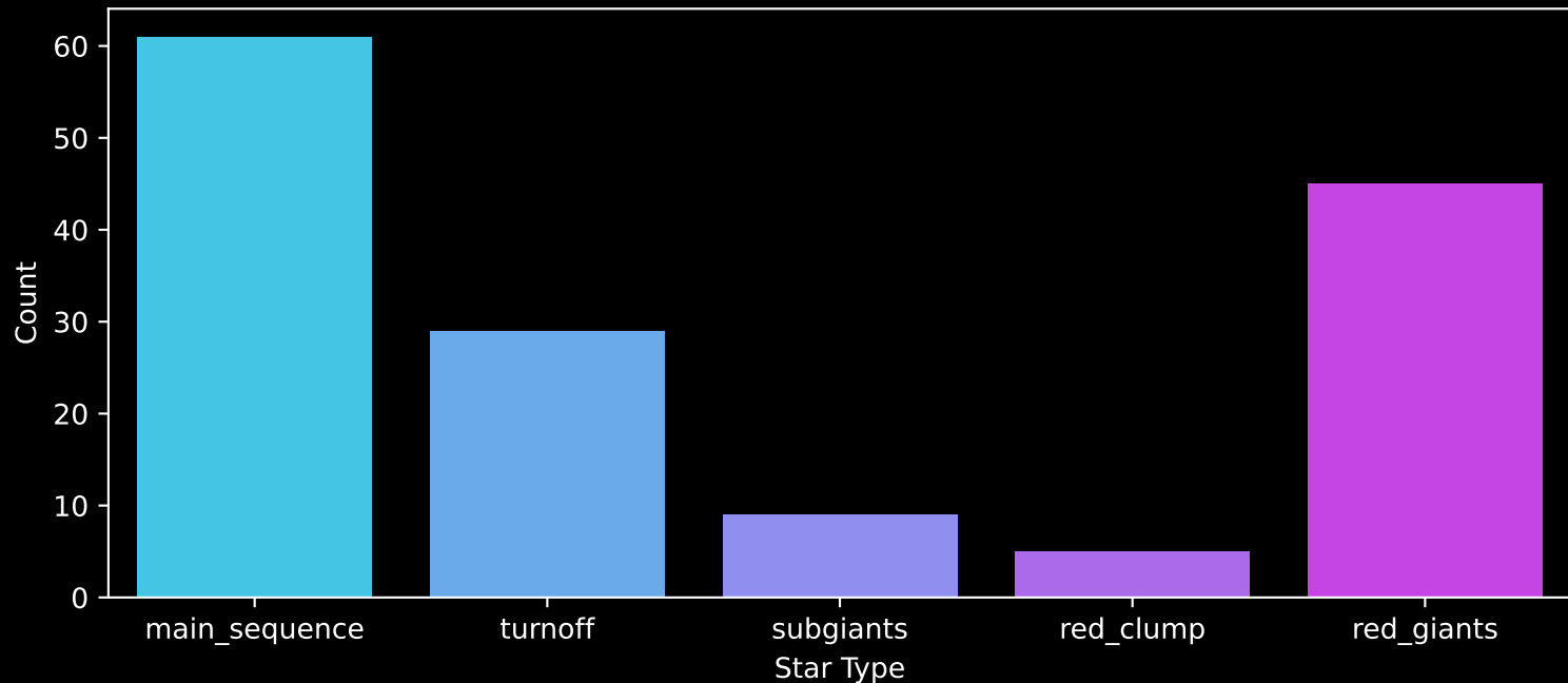
APOGEE DR17 Field: [042-31_MGA] Count plot of Star Type
