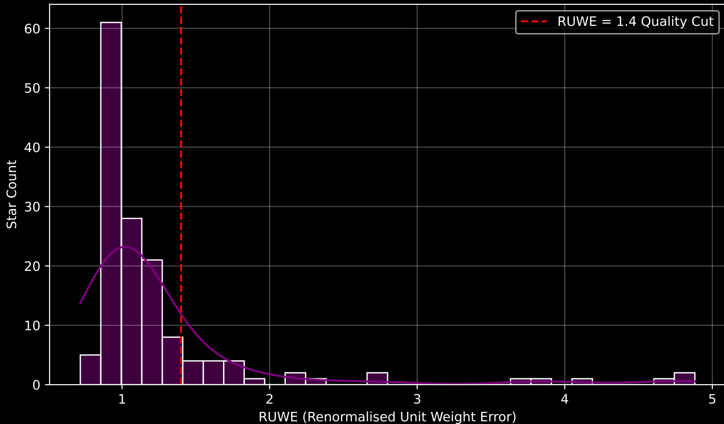
GAPOGEE DR17 Field [042-31_MGA] RUWE Distribution (n= 147)
