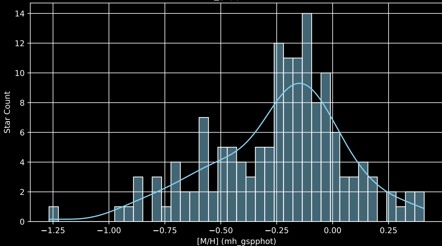
APOGEE DR17 Field: [042-31_MGA [M/H] (mh_gspphot) (n= 146)
