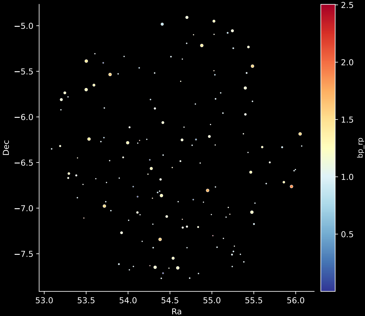
APOGEE DR17 Field: [042-31_MGA] Stars: 149
