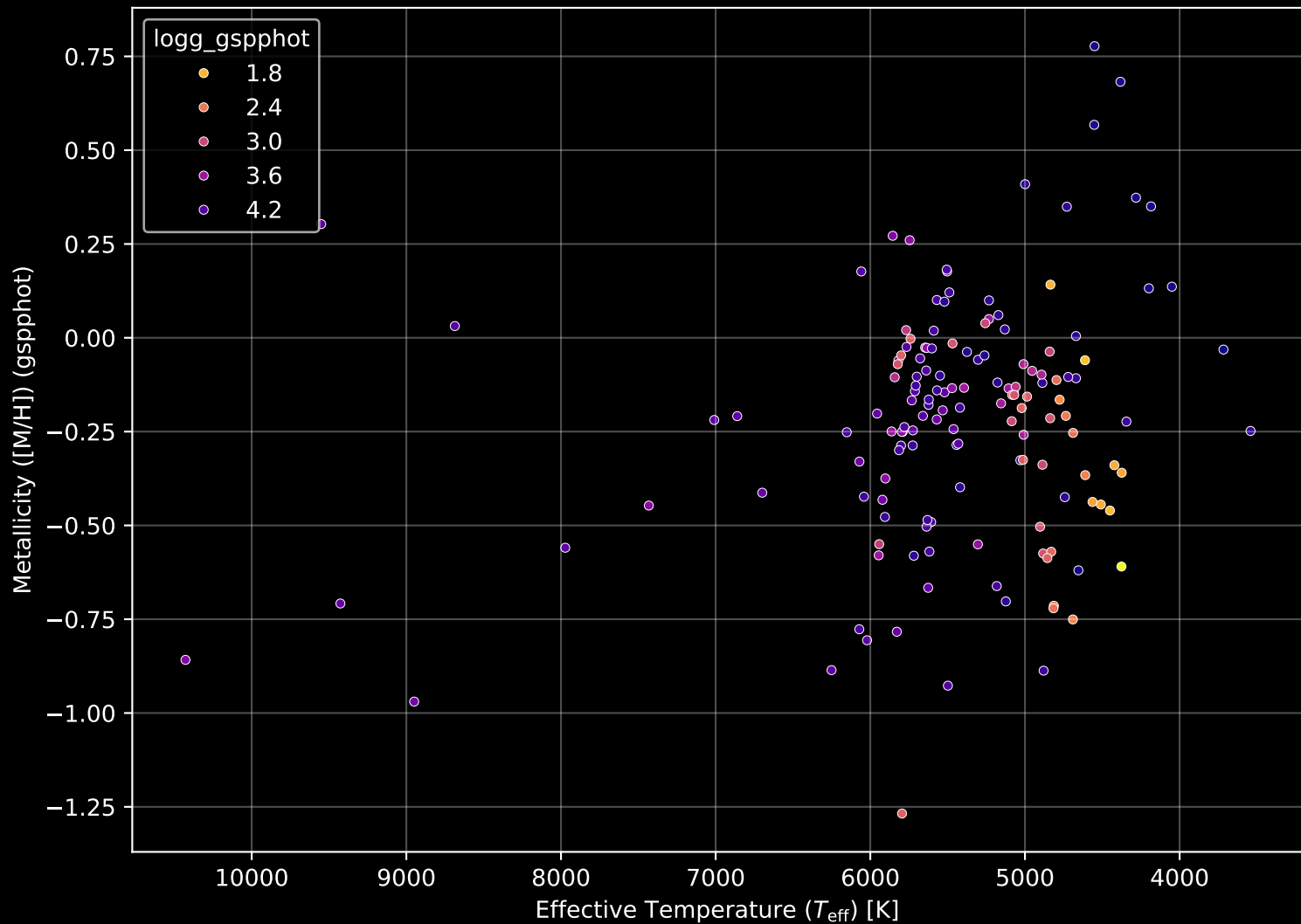
APOGEE DR17 Field: [042-31_MGA] Stellar Population Parameters (n= 149)
