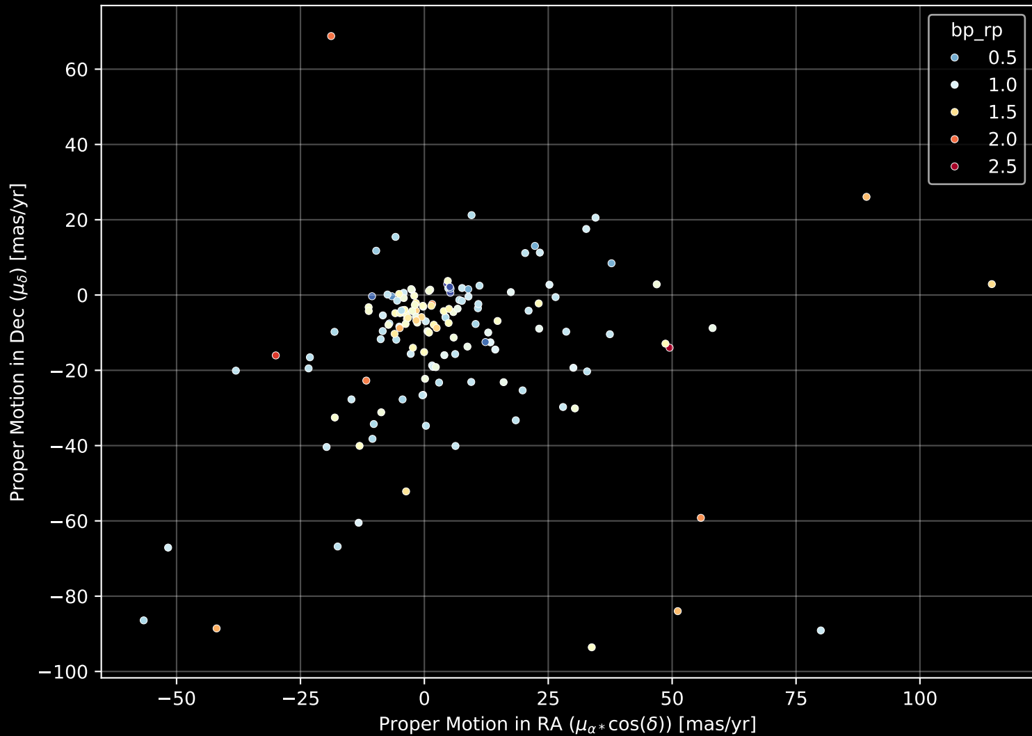
APOGEE DR17 Field: [042-31_MGA] Proper Motion Diagram (n= 149)
